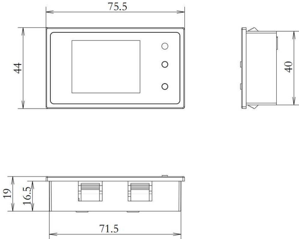
Dimension drawing
